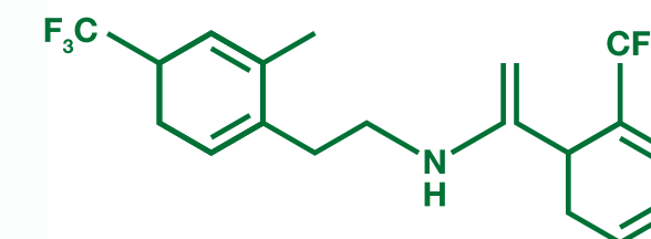
Fluopirame
